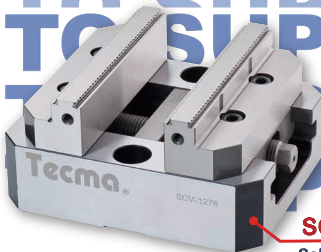
Self Centring Vise PAT.
